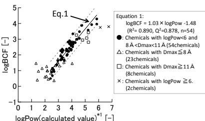
Fig.1 The relationship between logPow and logBCF for chemicals placed in Category I.
